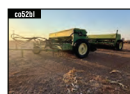
JOHN DEERE 8300 Stk# 5B, S/N 006816N, 20' Width, 2 GRAIN DRILLS, DOUBLE DRILL HITCH
