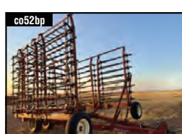
MCFARLANE HDL1036-16 Stk# 8F, 36" Width, 2" BAR, Spike Tooth 6-Flex Section Harrow 4" SPIKES, NICE!
